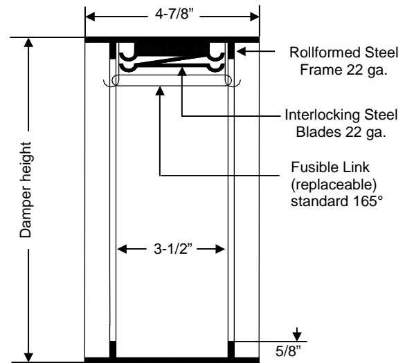
Vertical Section
